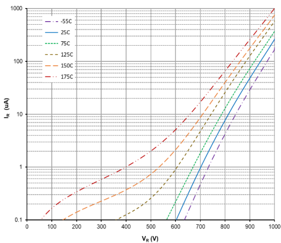
Figure 3. Reverse Characteristics
