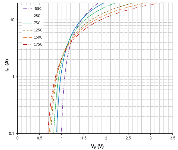
Figure 2. Forward Characteristics
